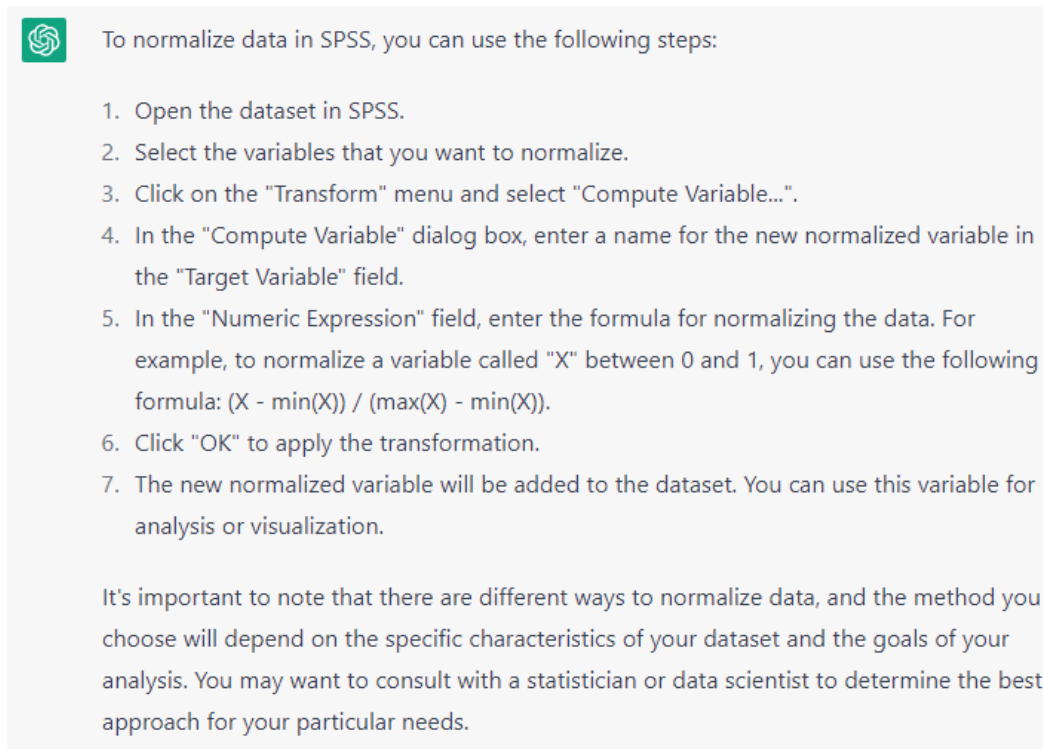
Fig. 5 The response of the CHAT-GPT-3 for the prompt "How can I normalize data in SPSS?"
